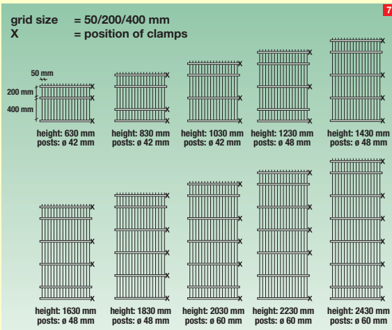
7. Fence heights and grid sizes
